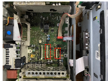
Check the installation position of the two Carplay flexible cables.
