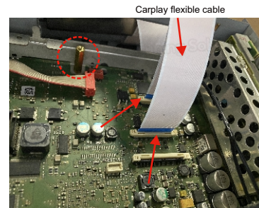
[1]. Check the direction of the blue part on the Carplay flexible cable. [2]. Check the copper post mounting position.
