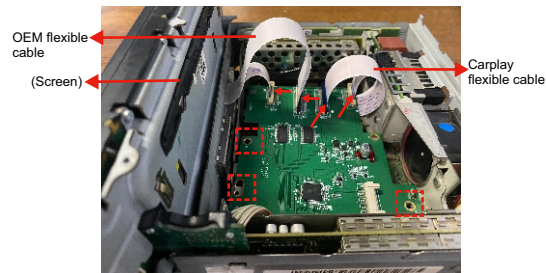
[1]. Check the Carplay flexible cable/OEM flexible cable installation position and the orientation of the blue part on the four soft cables Carplay flexible cable. [2]. Check the (3) screws mounting position.
