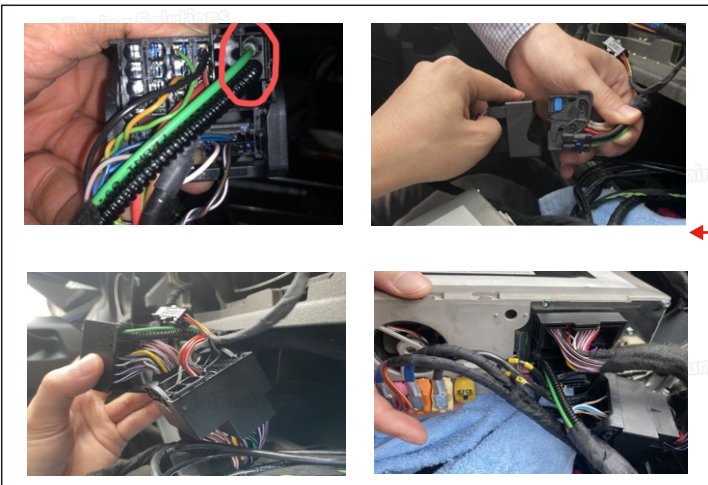
Adding a microphone: Disconnect and connect the additional microphone
